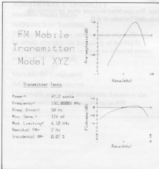
Figure 2-4. Example output of transmitter test program
